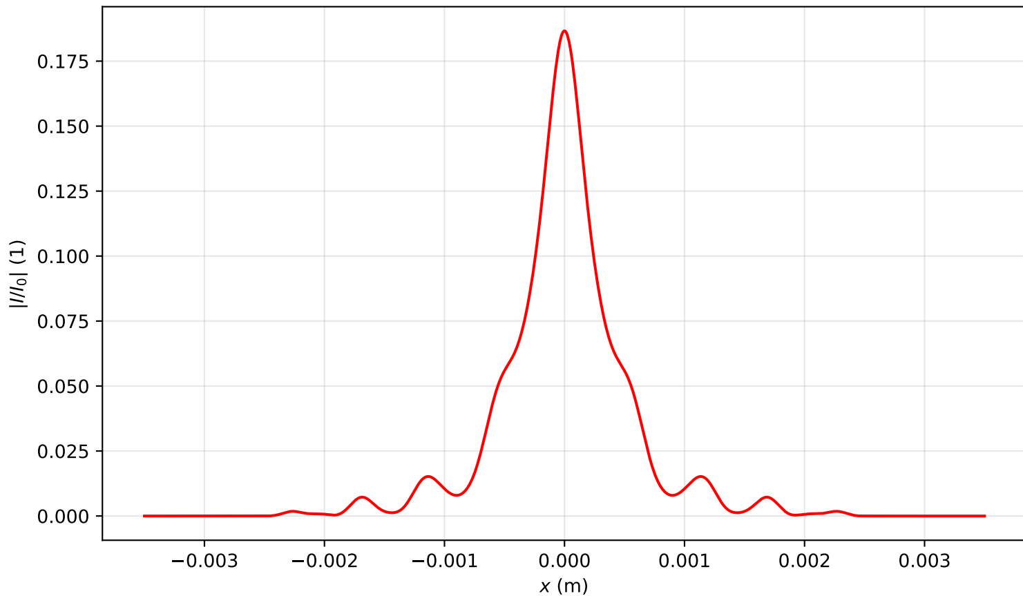
Intensity profile I(x, y = 0, z = 3.981)/I_0 , P_{in}=5.0P_{cr} , artificial time
